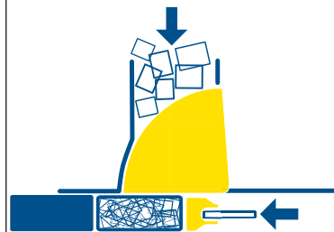
The main press compresses material with maximum pressure. The conveyor continues to feed material to the hopper.
