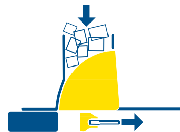
The strapping cycle begins when the preset bale length is reached. The main press continues in operation.
