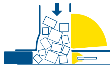
The pre-press and the main press in their starting positions. The press chamber is full.
